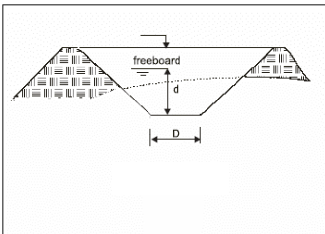
Figure 5.28: Channel design
