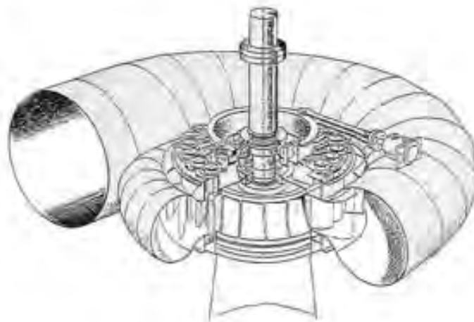
Figure 6.10: View of a Francis Turbine
