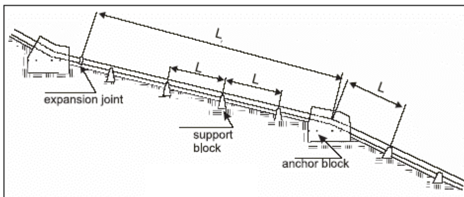
Figure 5.31: Penstock
