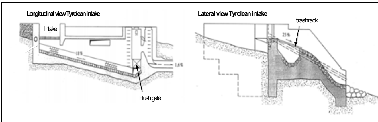
Figure 5.18: “Tyrolean” intake
