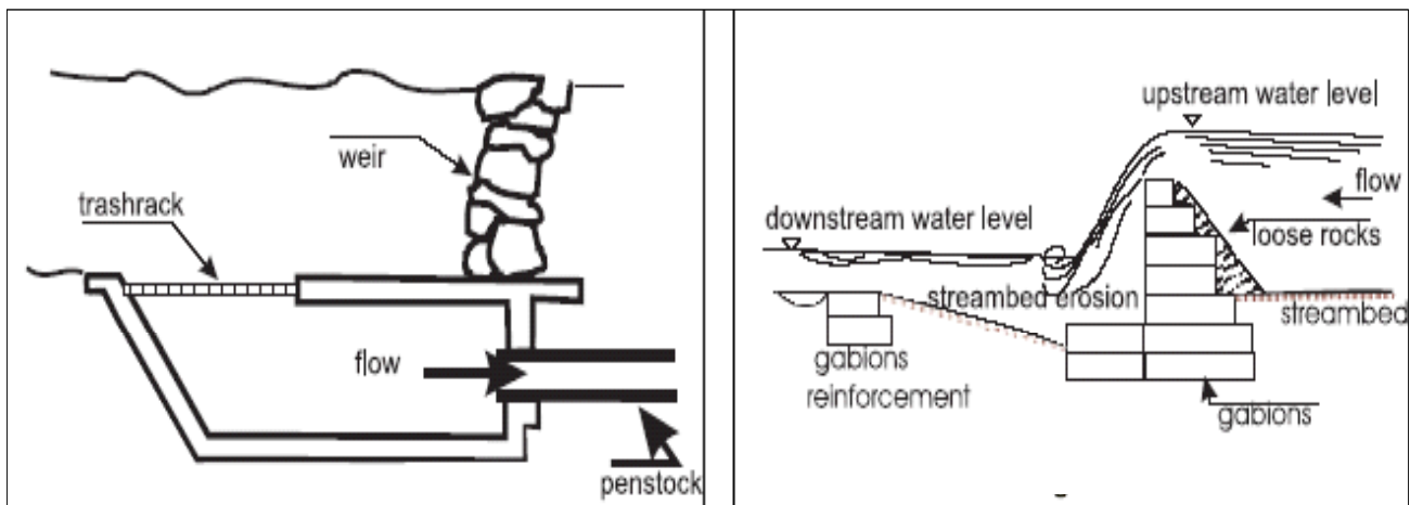
Figure 5.8: Weir configurations
