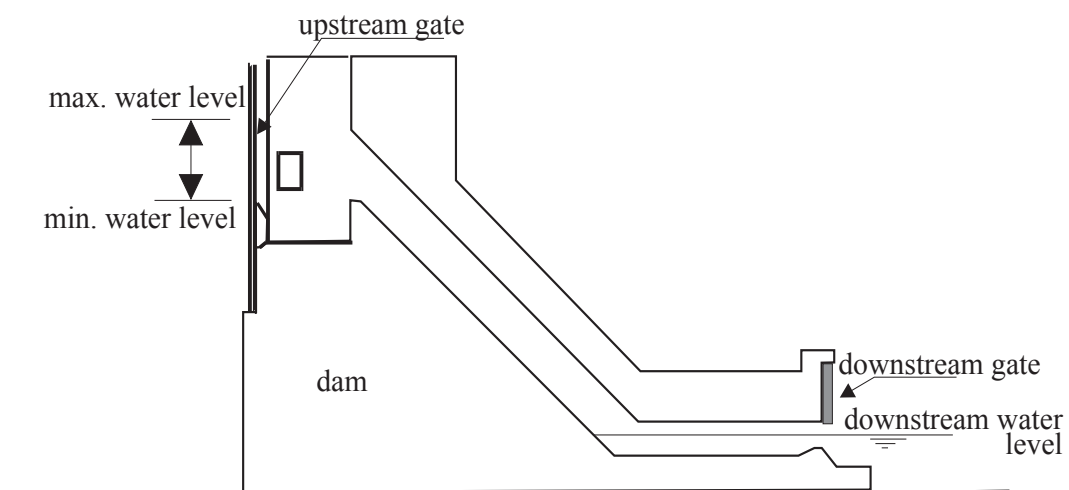
Figure 7.10: Section through Borland Lock
