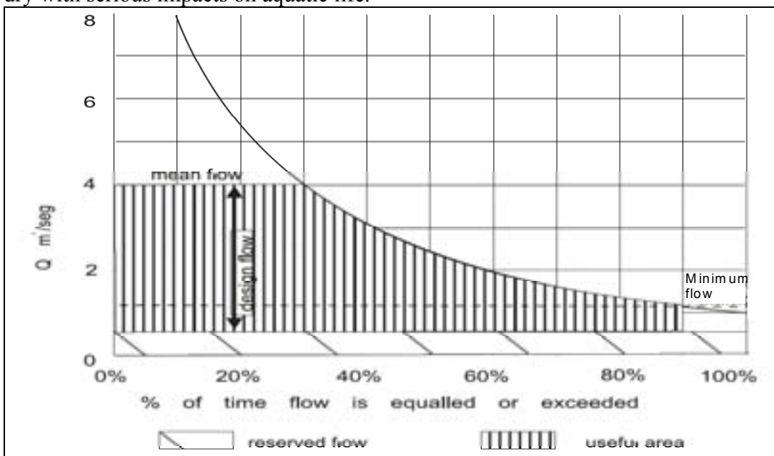
Figure 3-12 Residual flow
