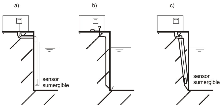
Figure 6.36 Level measurement
